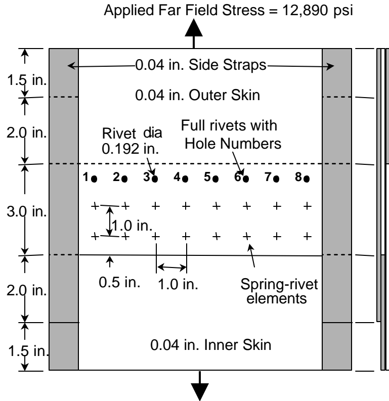
Figure 2. Configuration of NRC Lap Joint Specimens.
