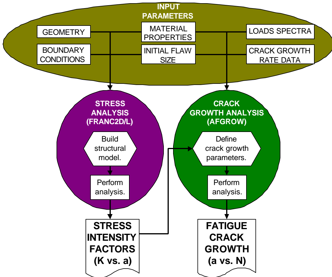
Figure 1. Analysis Tools for DTA of Riveted Lap Joints.
