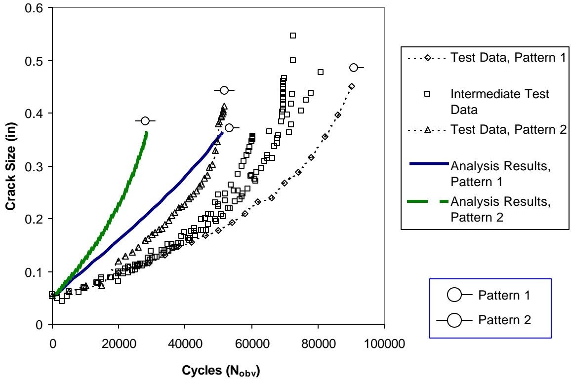
Figure 6. NRC Lap Joint Specimens Crack Growth Analysis and Test Results for Fatigue Specimens.
